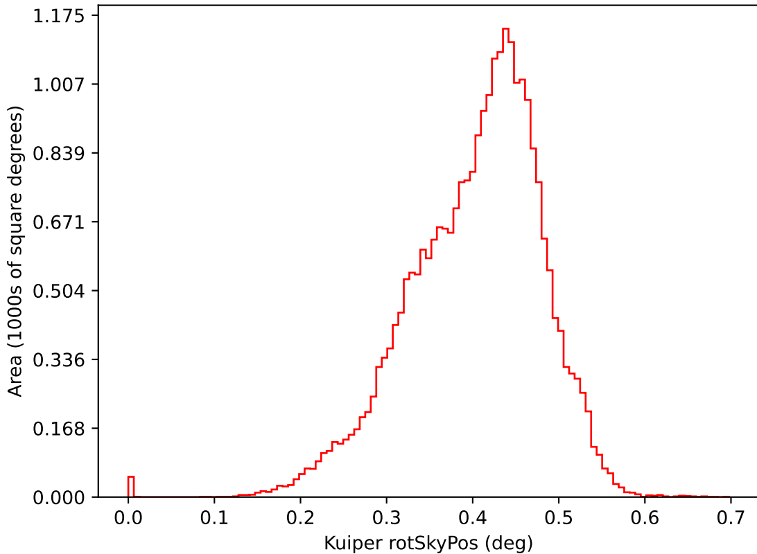
too_elab_r8_d3_griz_v3.4_10yrs i: Kuiper rotSkyPos
