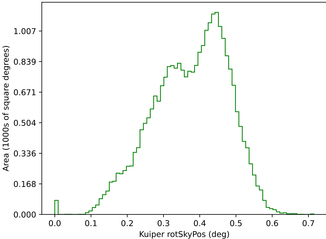
too_elab_r8_d3_griz_v3.4_10yrs g: Kuiper rotSkyPos
