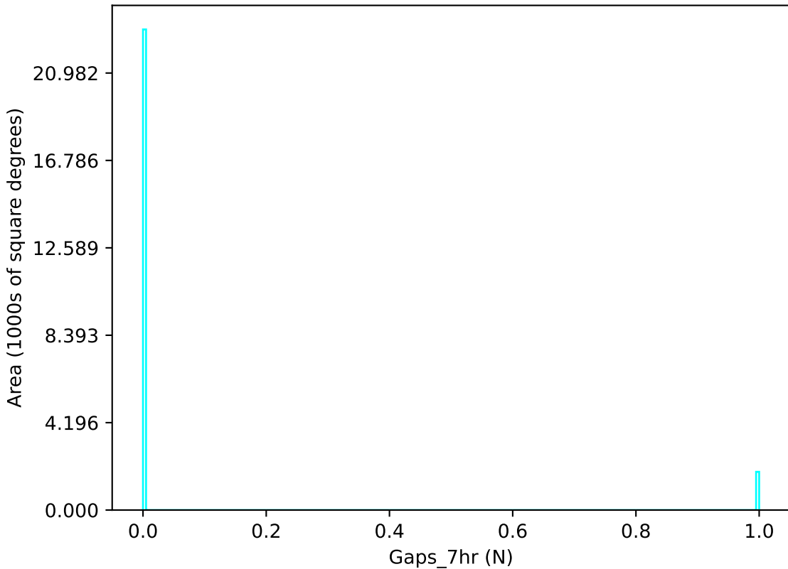
too_elab_r8_d3_griz_v3.4_10yrs u band: Gaps_7hr
