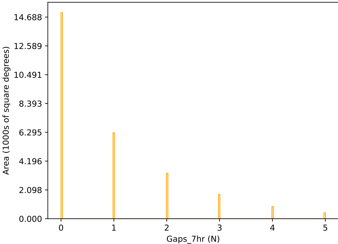
too_elab_r8_d3_griz_v3.4_10yrs r band: Gaps_7hr
