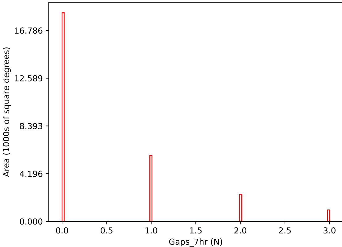
too_elab_r8_d3_griz_v3.4_10yrs i band: Gaps_7hr
