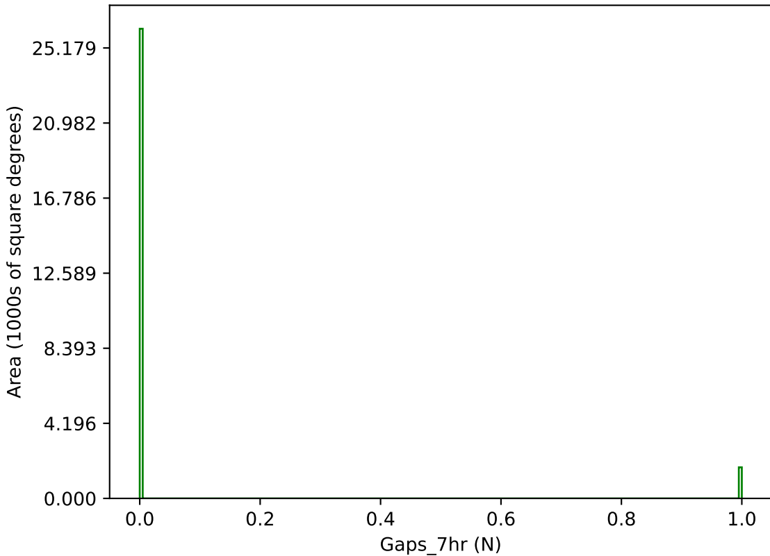
too_elab_r8_d3_griz_v3.4_10yrs g band: Gaps_7hr
