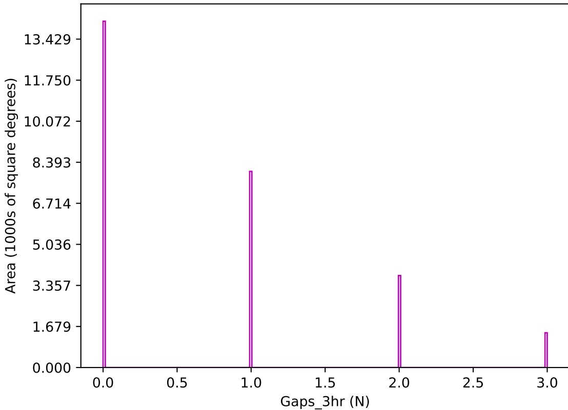
too_elab_r8_d3_griz_v3.4_10yrs z band: Gaps_3hr
