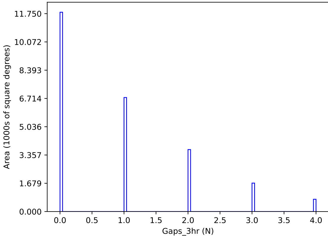
too_elab_r8_d3_griz_v3.4_10yrs y band: Gaps_3hr
