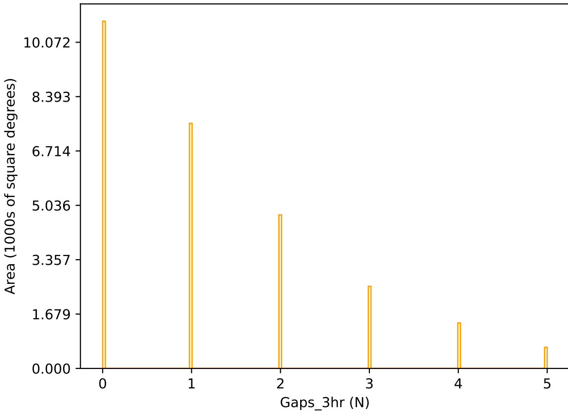
too_elab_r8_d3_griz_v3.4_10yrs r band: Gaps_3hr
