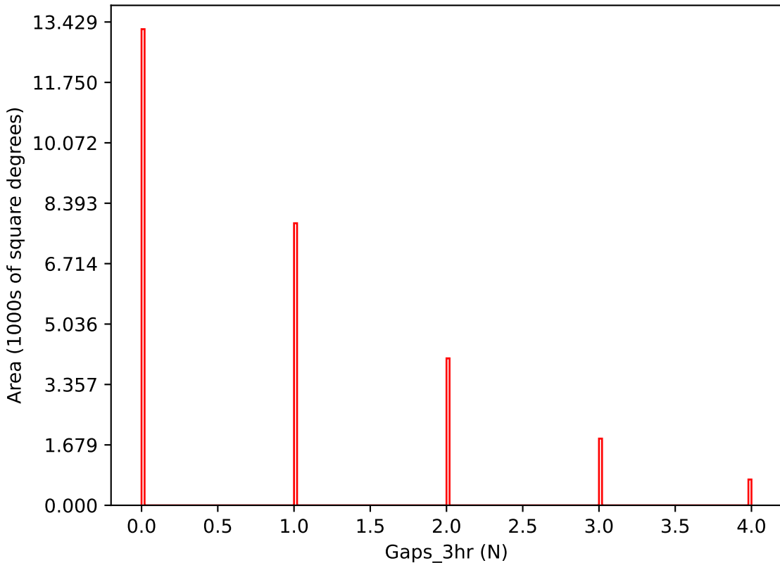
too_elab_r8_d3_griz_v3.4_10yrs i band: Gaps_3hr
