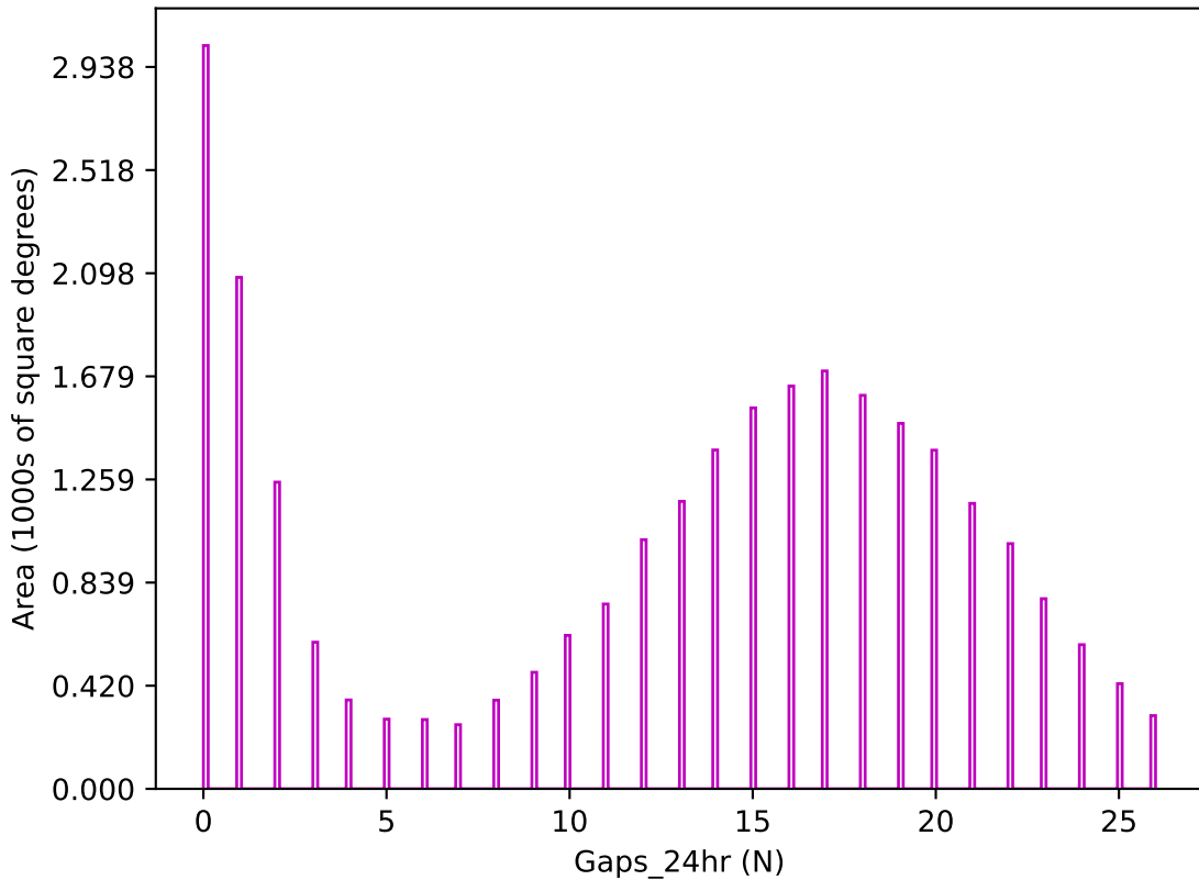
too_elab_r8_d3_griz_v3.4_10yrs z band: Gaps_24hr
