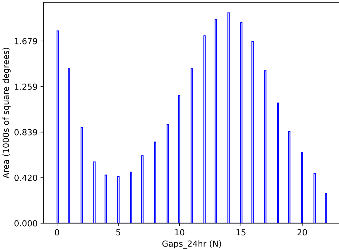
too_elab_r8_d3_griz_v3.4_10yrs y band: Gaps_24hr
