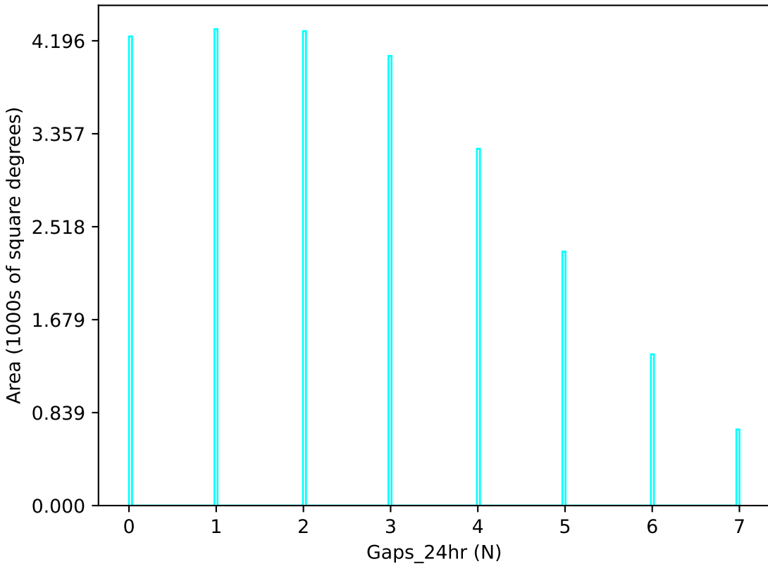
too_elab_r8_d3_griz_v3.4_10yrs u band: Gaps_24hr
