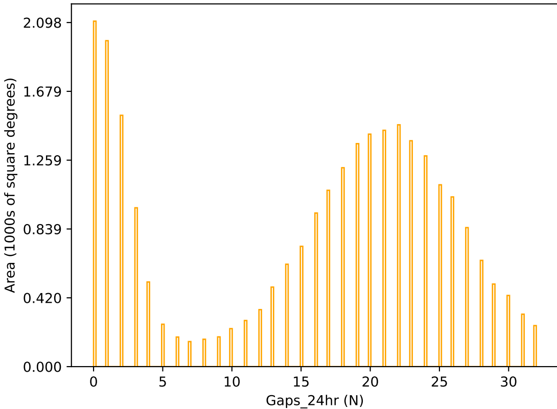
too_elab_r8_d3_griz_v3.4_10yrs r band: Gaps_24hr
