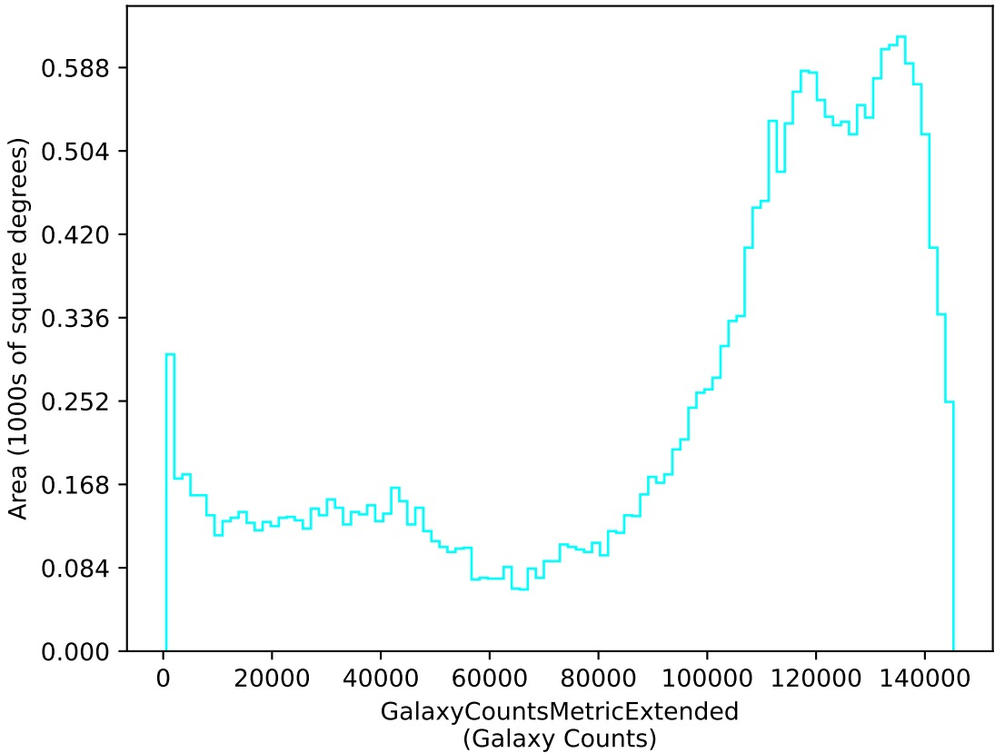
too_elab_r8_d3_griz_v3.4_10yrs u: GalaxyCountsMetricExtended
