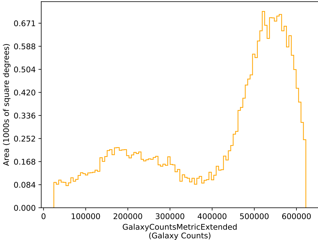
too_elab_r8_d3_griz_v3.4_10yrs r: GalaxyCountsMetricExtended
