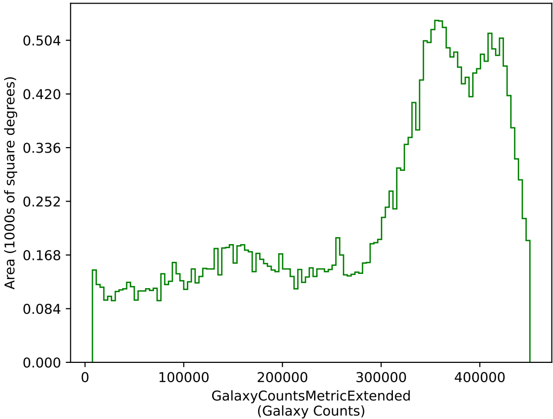
too_elab_r8_d3_griz_v3.4_10yrs g: GalaxyCountsMetricExtended
