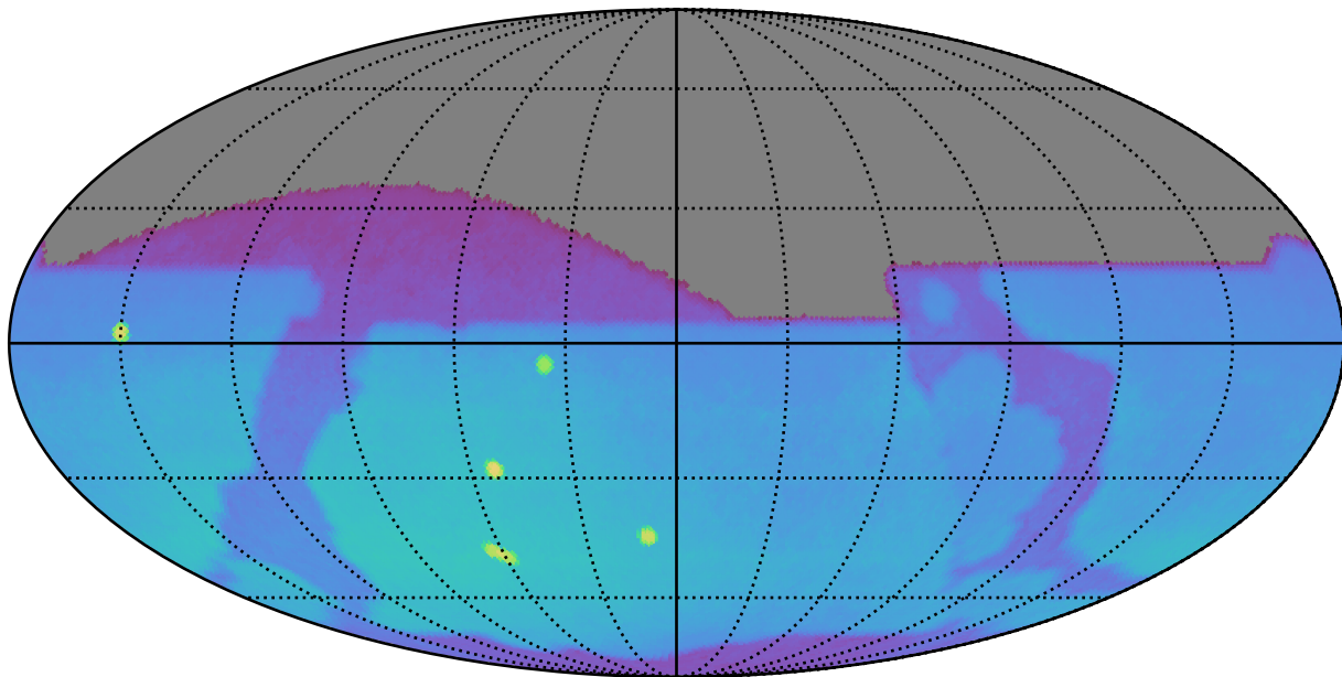
too_elab_r8_d3_griz_v3.4_10yrs : Brown Dwarf, L7
