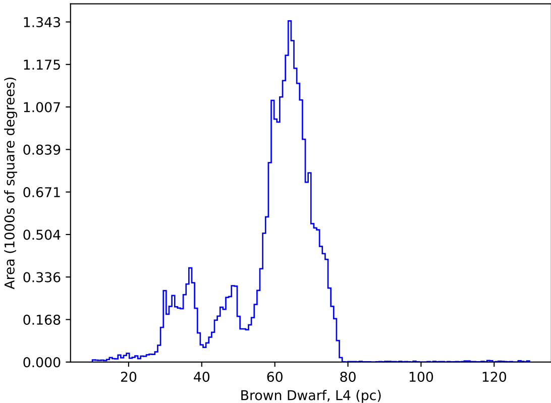
too_elab_r8_d3_griz_v3.4_10yrs : Brown Dwarf, L4
