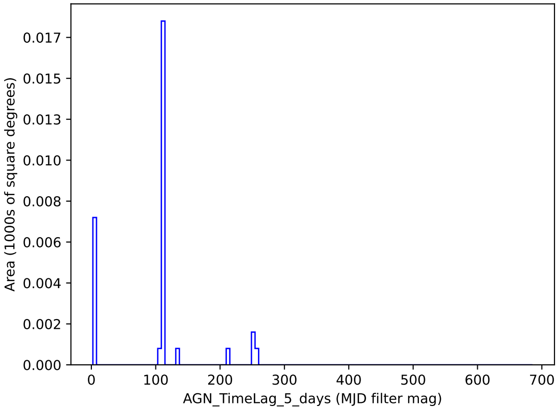
too_elab_r8_d3_griz_v3.4_10yrs y band: AGN_TimeLag_5_days
