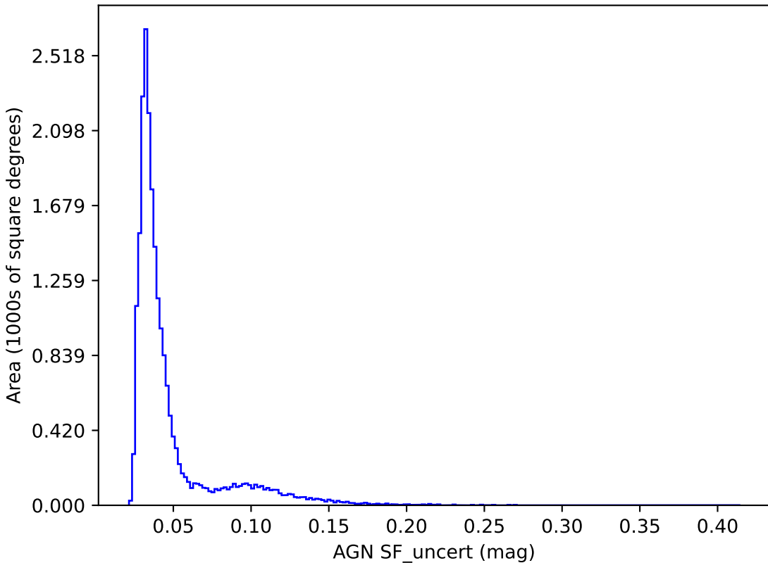
too_elab_r8_d3_griz_v3.4_10yrs y band: AGN SF_uncert
