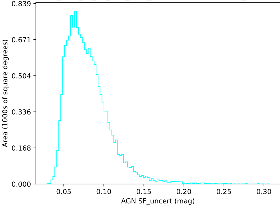
too_elab_r8_d3_griz_v3.4_10yrs u band: AGN SF_uncert
