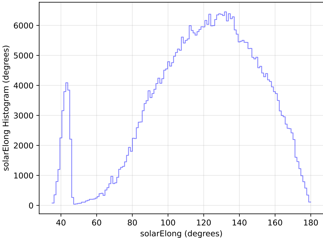
too_elab_r8_d3_griz_v3.4_10yrs WFD z band: solarElong Histogram
