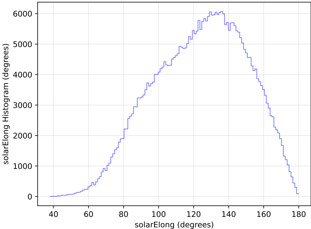
too_elab_r8_d3_griz_v3.4_10yrs WFD y band: solarElong Histogram
