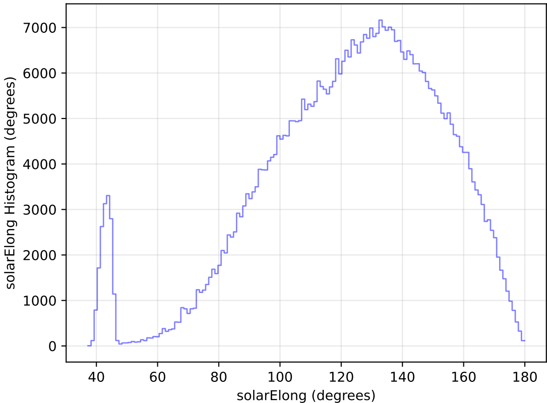
too_elab_r8_d3_griz_v3.4_10yrs WFD r band: solarElong Histogram
