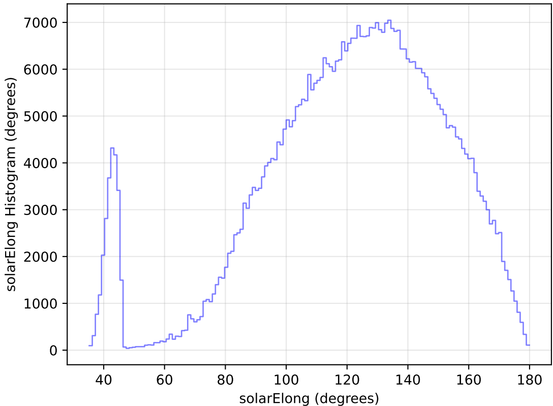
too_elab_r8_d3_griz_v3.4_10yrs WFD i band: solarElong Histogram
