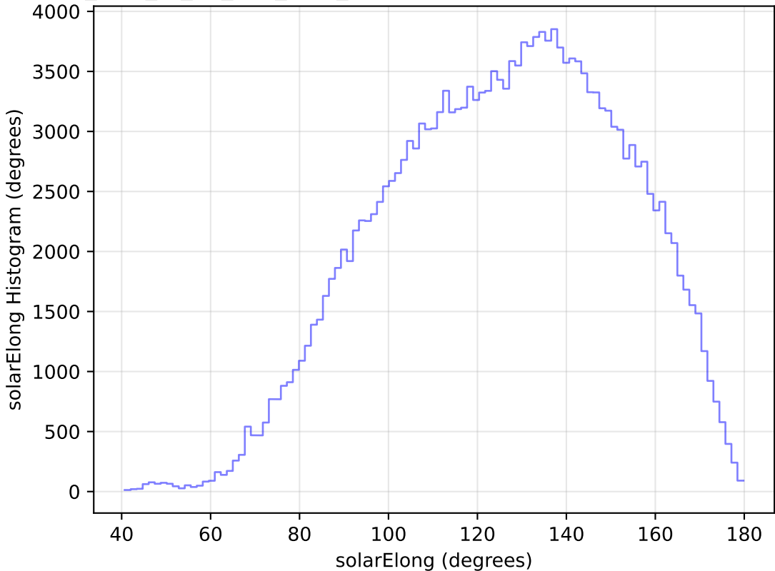
too_elab_r8_d3_griz_v3.4_10yrs WFD g band: solarElong Histogram
