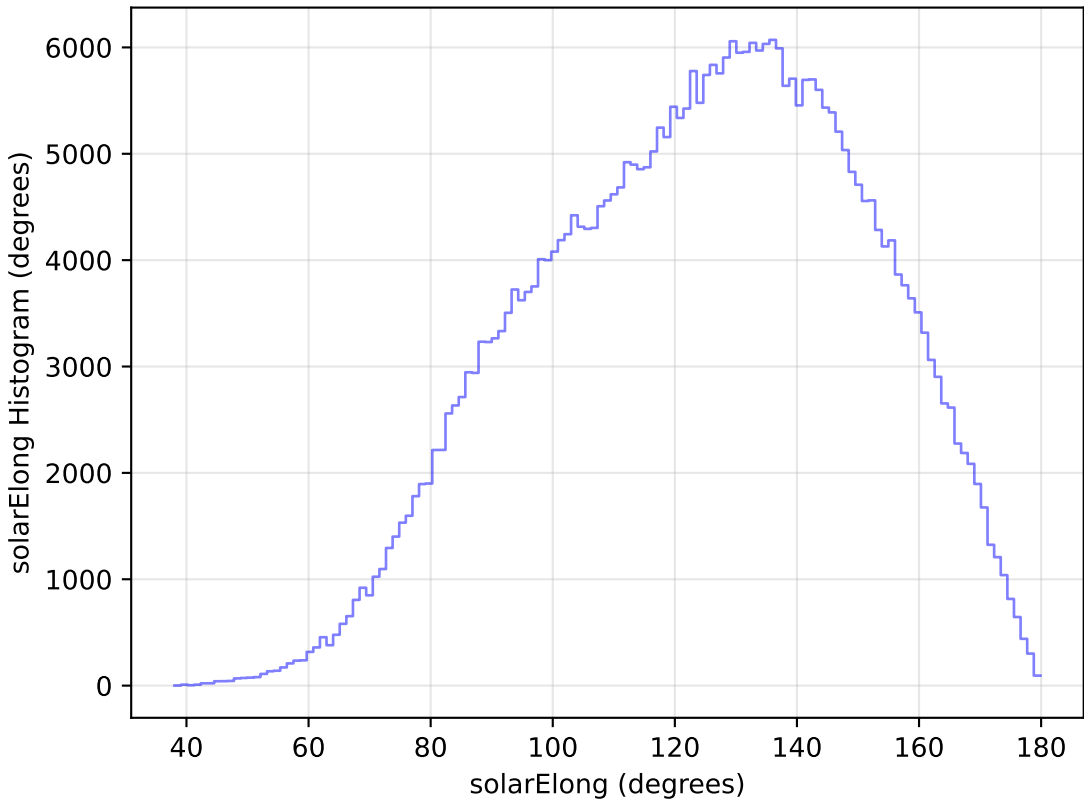
too_elab_r8_d3_griz_v3.4_10yrs All sky y band: solarElong Histogram
