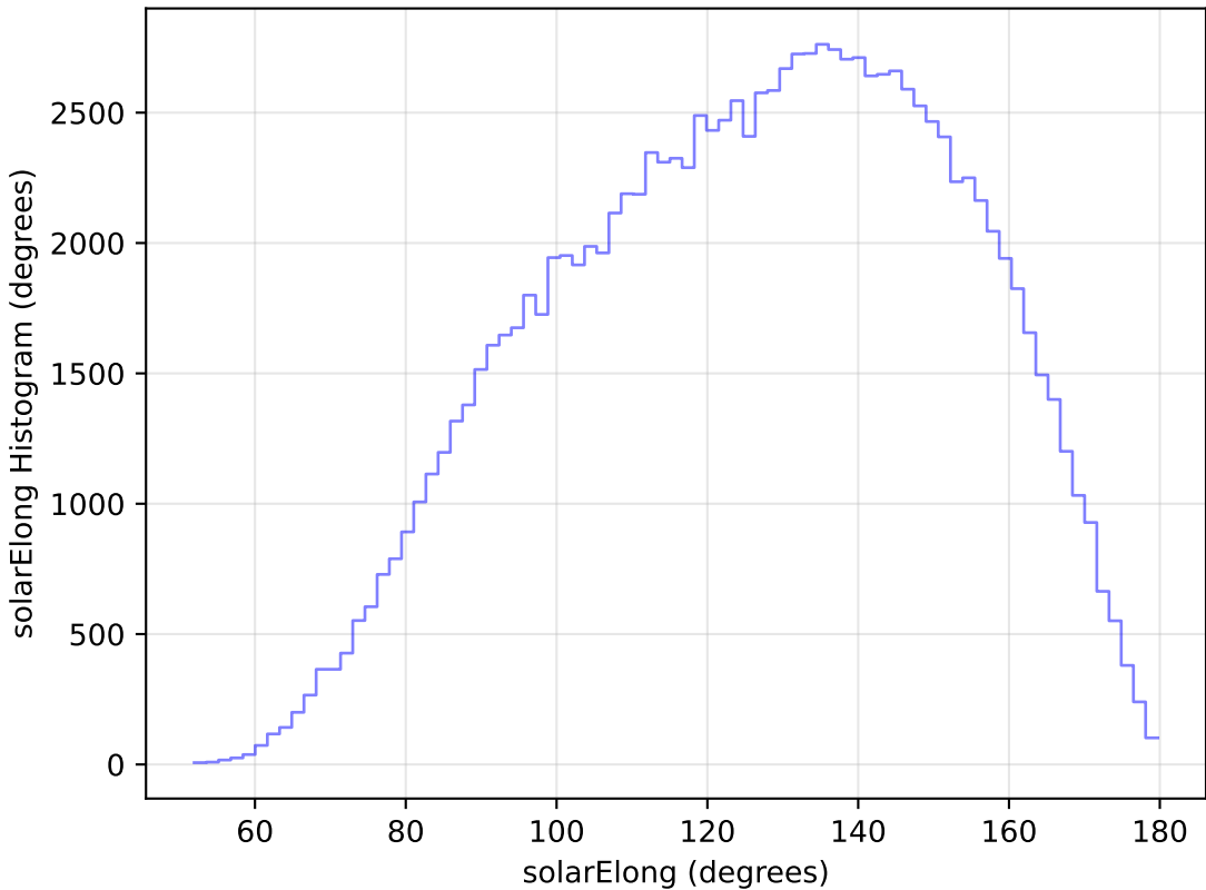
too_elab_r8_d3_griz_v3.4_10yrs All sky u band: solarElong Histogram
