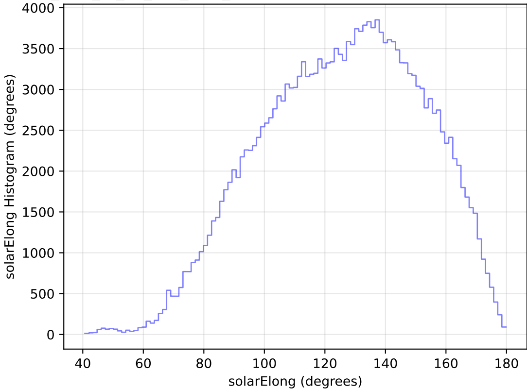
too_elab_r8_d3_griz_v3.4_10yrs All sky g band: solarElong Histogram
