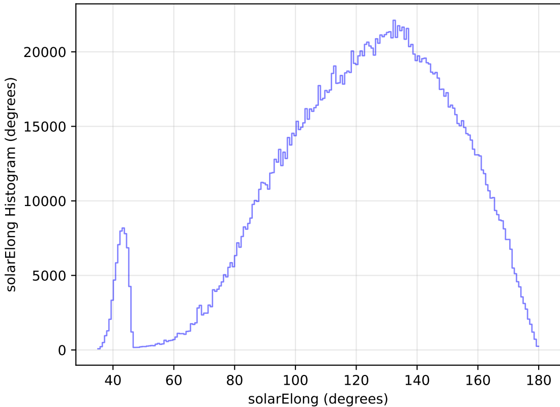
too_elab_r8_d3_griz_v3.4_10yrs All sky all bands: solarElong Histogram
