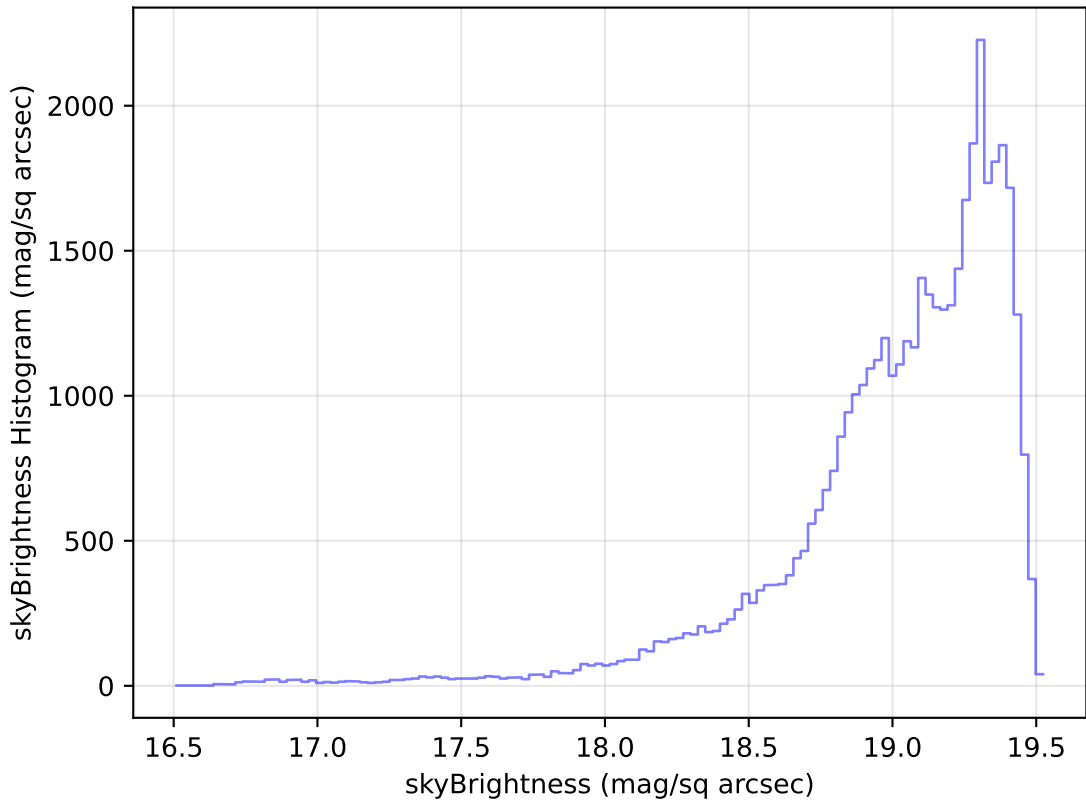
too_elab_r8_d3_griz_v3.4_10yrs Yr 1 z band: skyBrightness Histogram
