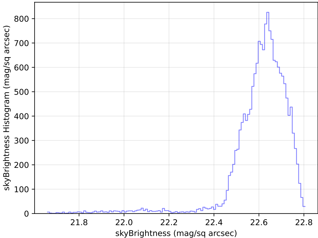
too_elab_r8_d3_griz_v3.4_10yrs Yr 1 u band: skyBrightness Histogram
