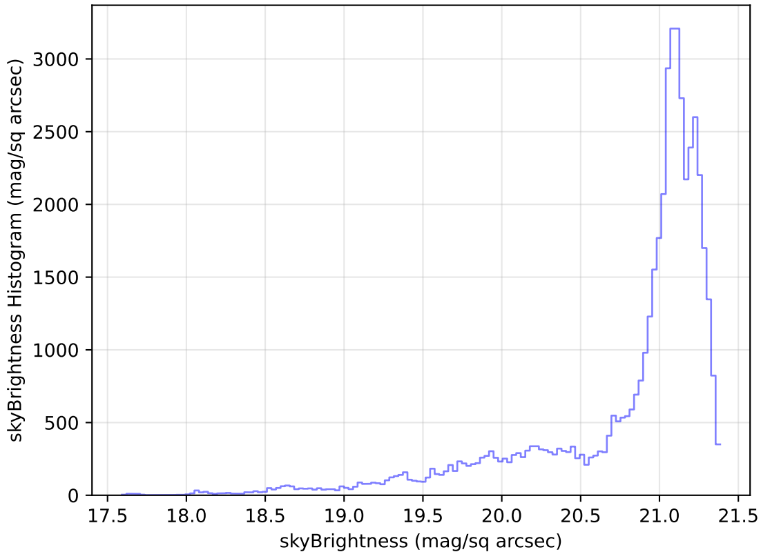
too_elab_r8_d3_griz_v3.4_10yrs Yr 1 r band: skyBrightness Histogram
