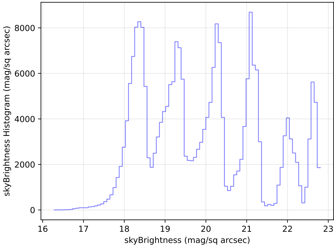
too_elab_r8_d3_griz_v3.4_10yrs Yr 1 all bands: skyBrightness Histogram
