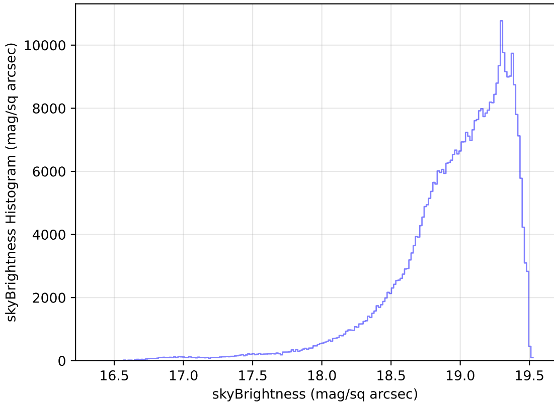
too_elab_r8_d3_griz_v3.4_10yrs WFD z band: skyBrightness Histogram
