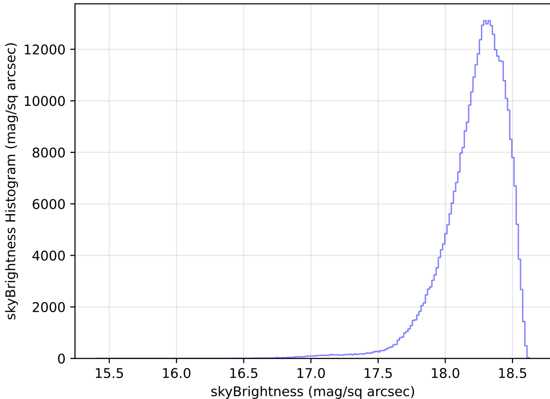
too_elab_r8_d3_griz_v3.4_10yrs WFD y band: skyBrightness Histogram
