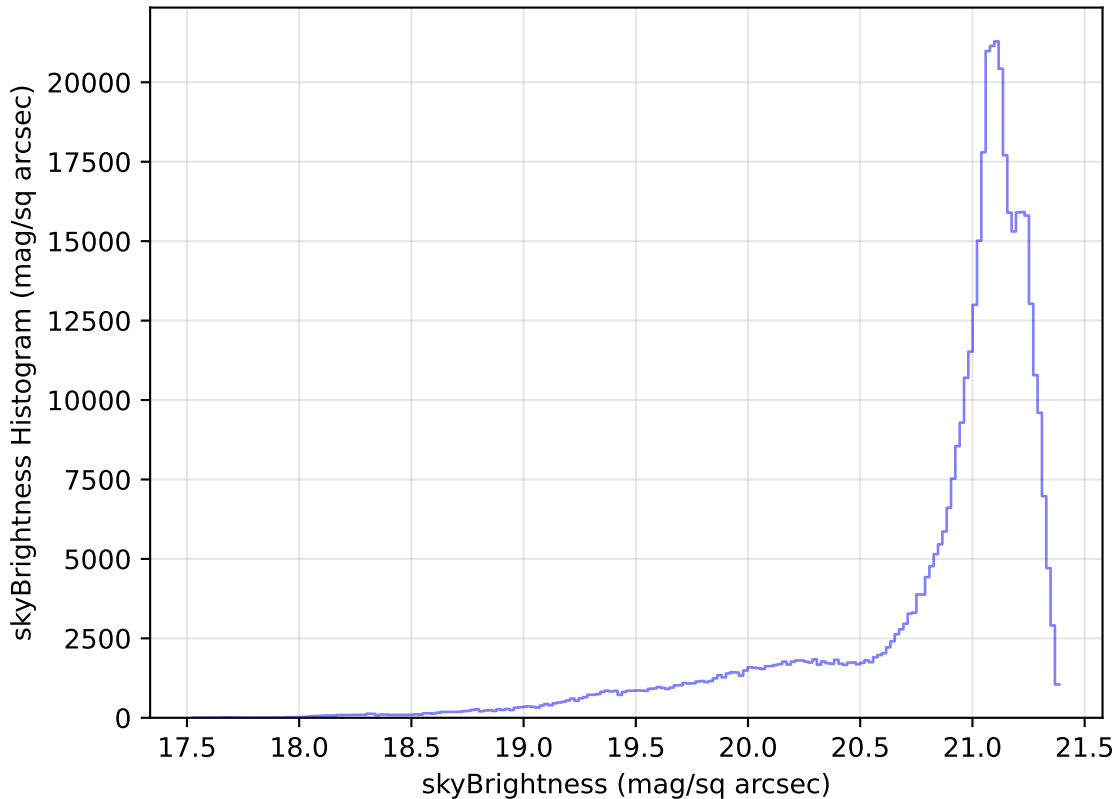
too_elab_r8_d3_griz_v3.4_10yrs WFD r band: skyBrightness Histogram
