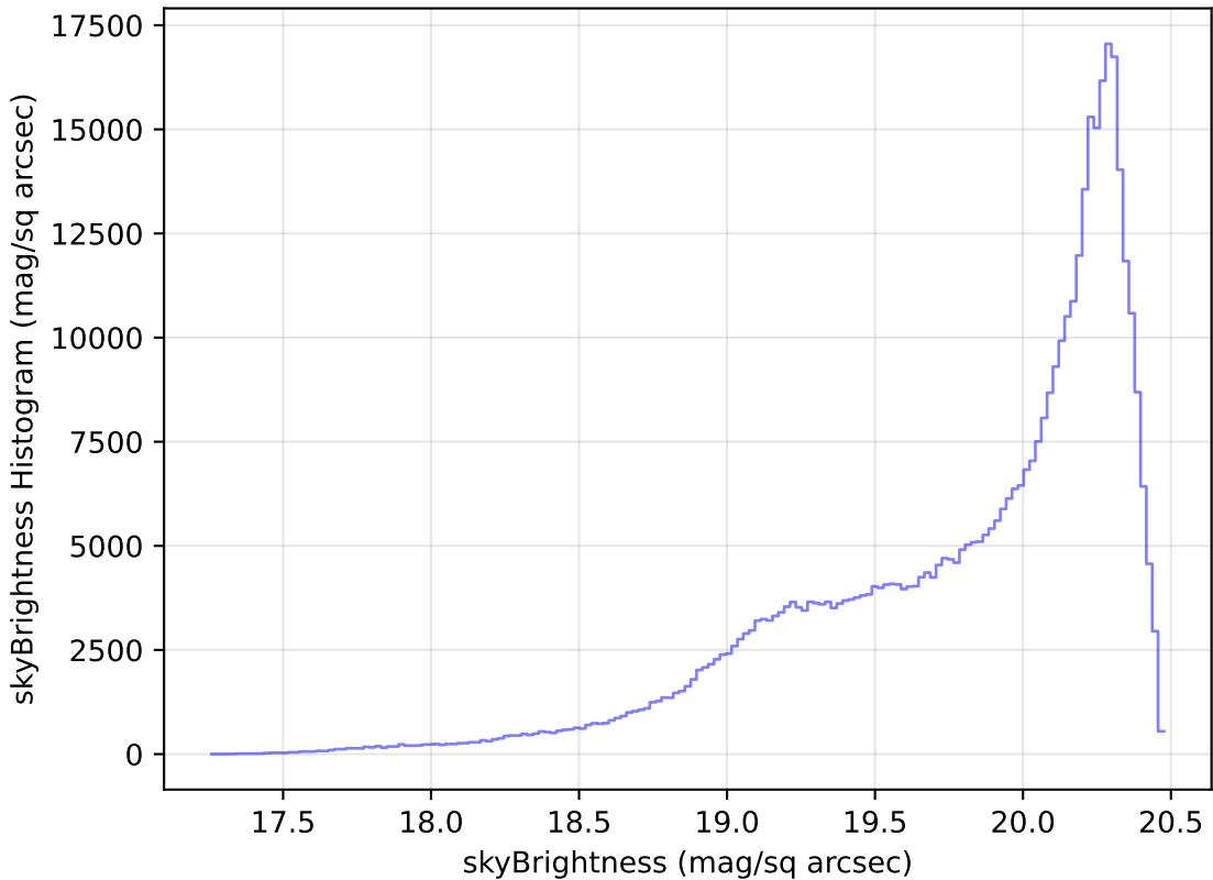
too_elab_r8_d3_griz_v3.4_10yrs WFD i band: skyBrightness Histogram
