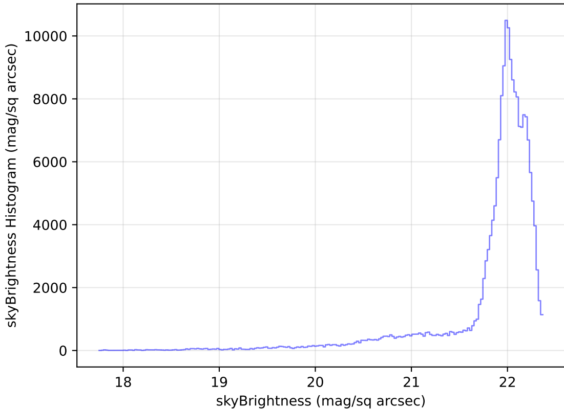
too_elab_r8_d3_griz_v3.4_10yrs WFD g band: skyBrightness Histogram
