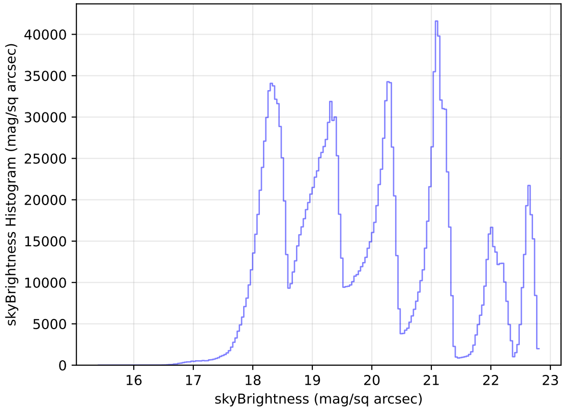
too_elab_r8_d3_griz_v3.4_10yrs WFD all bands: skyBrightness Histogram
