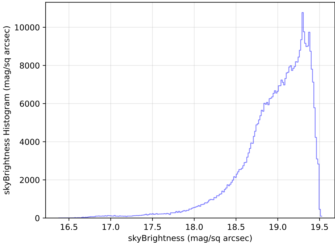
too_elab_r8_d3_griz_v3.4_10yrs All sky z band: skyBrightness Histogram
