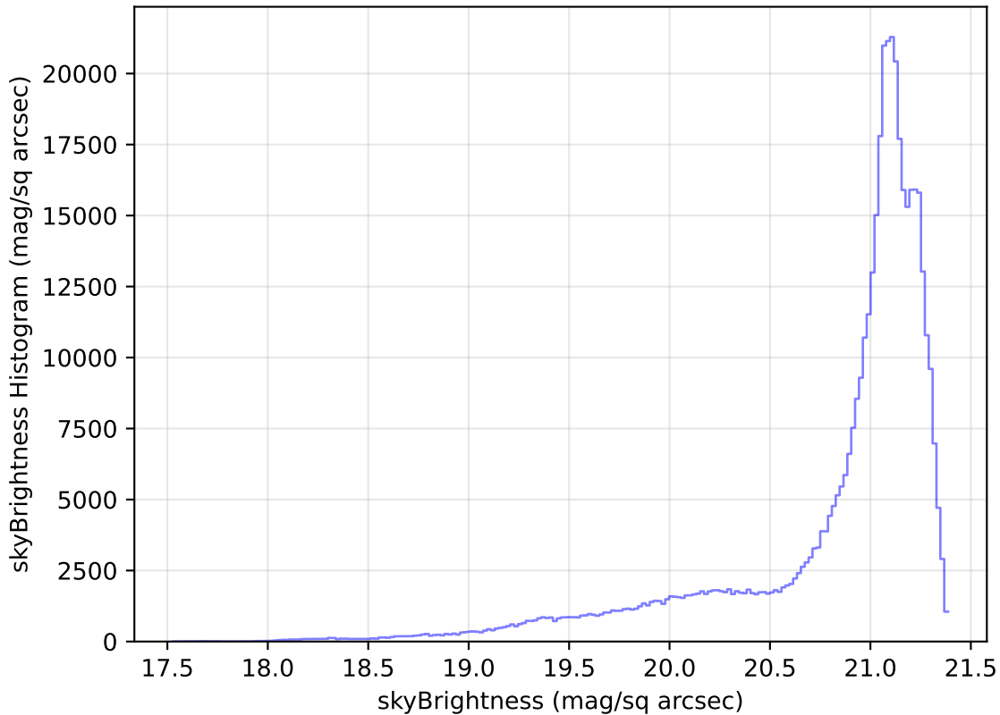
too_elab_r8_d3_griz_v3.4_10yrs All sky r band: skyBrightness Histogram
