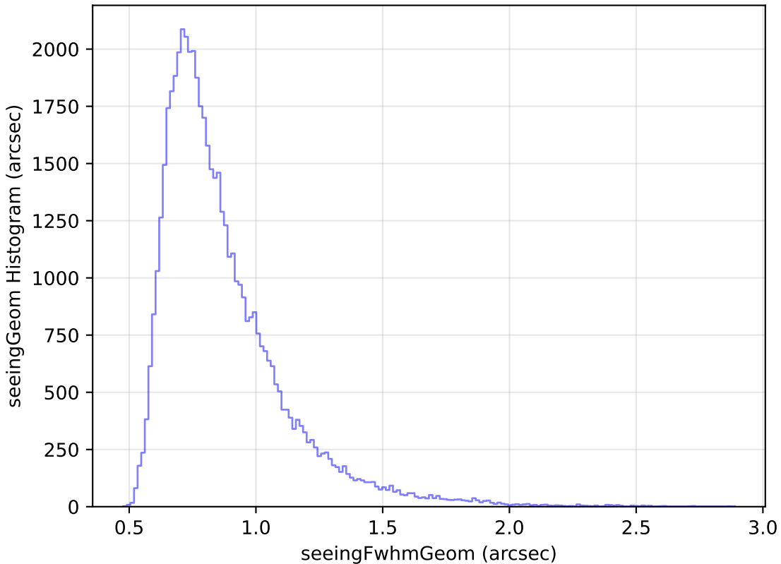
too_elab_r8_d3_griz_v3.4_10yrs Yr 1 i band: seeingGeom Histogram
