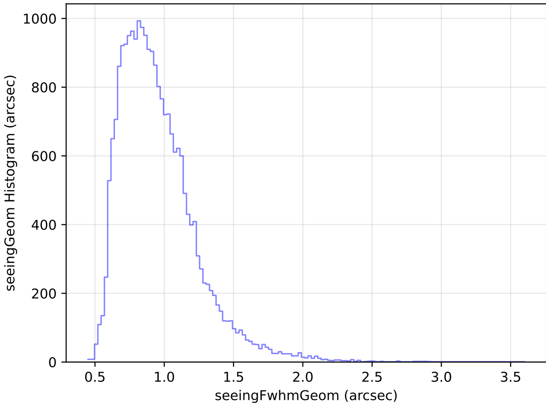
too_elab_r8_d3_griz_v3.4_10yrs Yr 1 g band: seeingGeom Histogram
