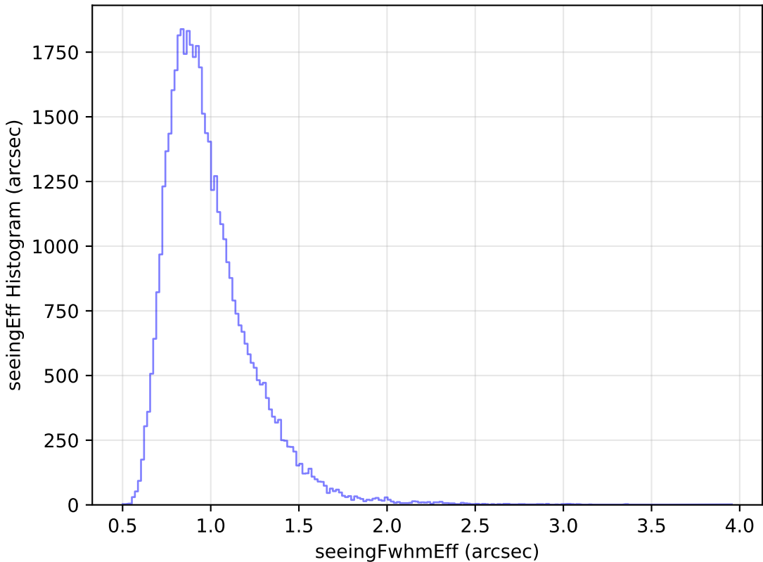
too_elab_r8_d3_griz_v3.4_10yrs Yr 1 y band: seeingEff Histogram
