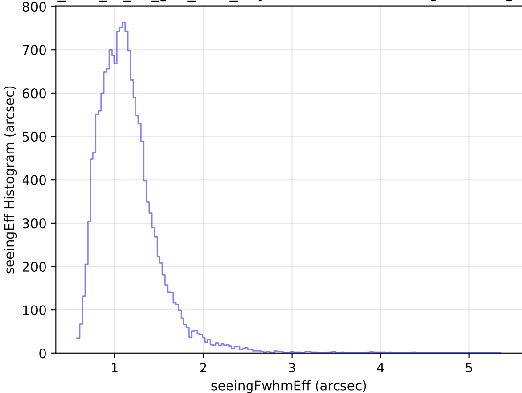
too_elab_r8_d3_griz_v3.4_10yrs Yr 1 u band: seeingEff Histogram
