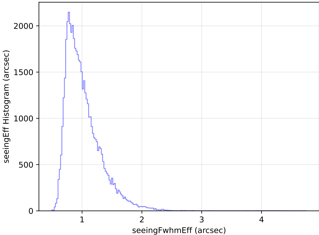
too_elab_r8_d3_griz_v3.4_10yrs Yr 1 r band: seeingEff Histogram
