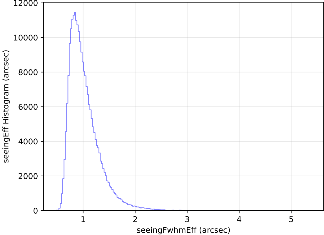
too_elab_r8_d3_griz_v3.4_10yrs Yr 1 all bands: seeingEff Histogram
