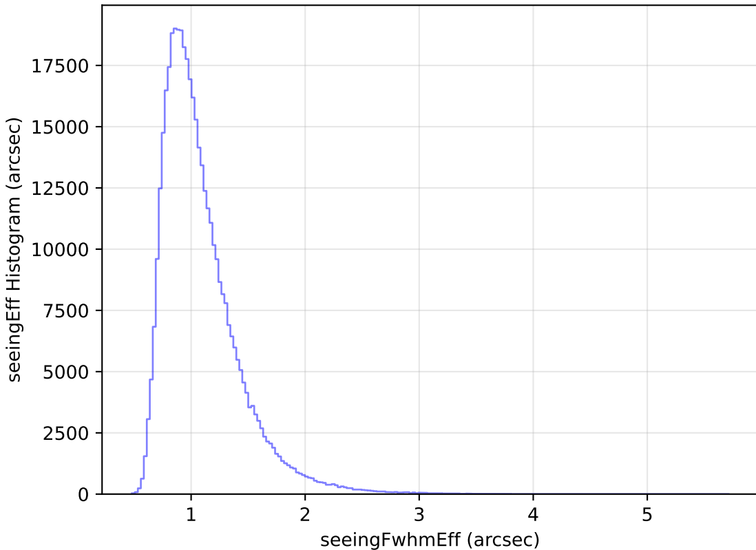
too_elab_r8_d3_griz_v3.4_10yrs WFD z band: seeingEff Histogram
